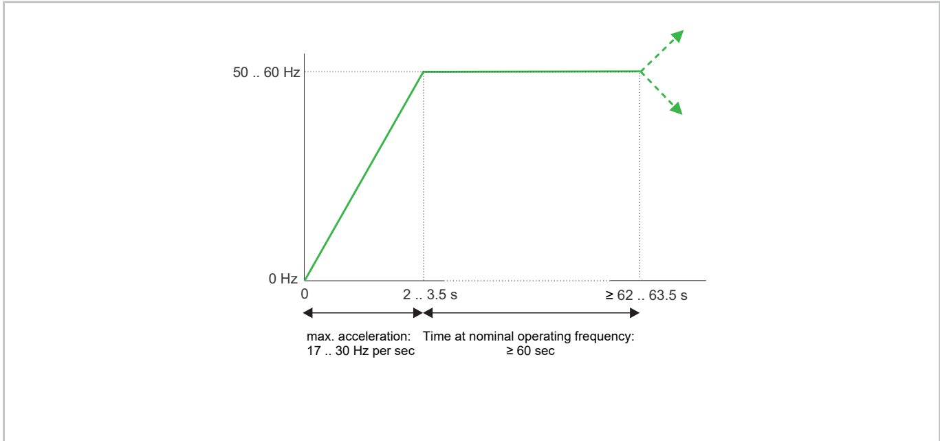
Fig. 16: Exemplary start sequence for ORBIT and ESH7 scroll compressors with frequency inverter.
