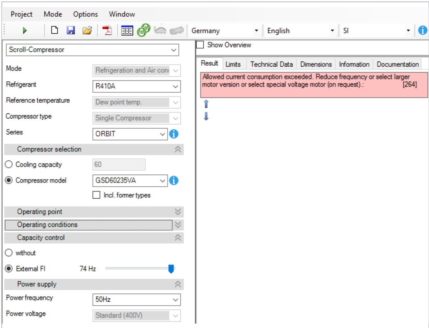
Fig. 6: By increasing the operating frequency of the selected compressor, the maximum current consumption may be exceeded. In this case, the software recommends e.g. a special voltage motor.
