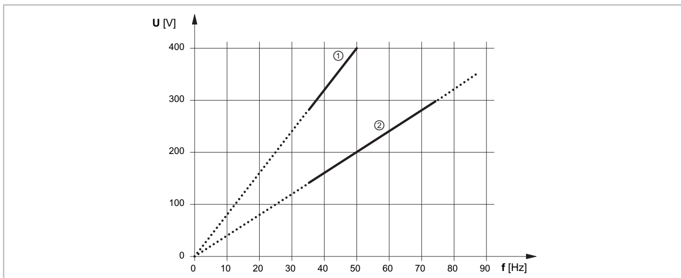
Fig. 14: Voltage increase of an ORBIT compressor (E..7 series: max 65 Hz), depending on the frequency for different motors
