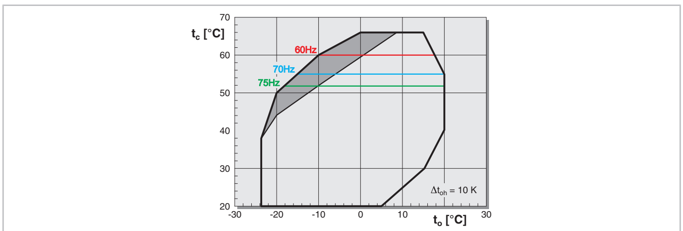
Fig. 4: Exemplary and simplified application limits for an ORBIT scroll compressor with frequency inverter at 60, 70 and 75 Hz (limits due to motor temperature or maximum current). The compressor may only be operated below the indicated frequency lines.
