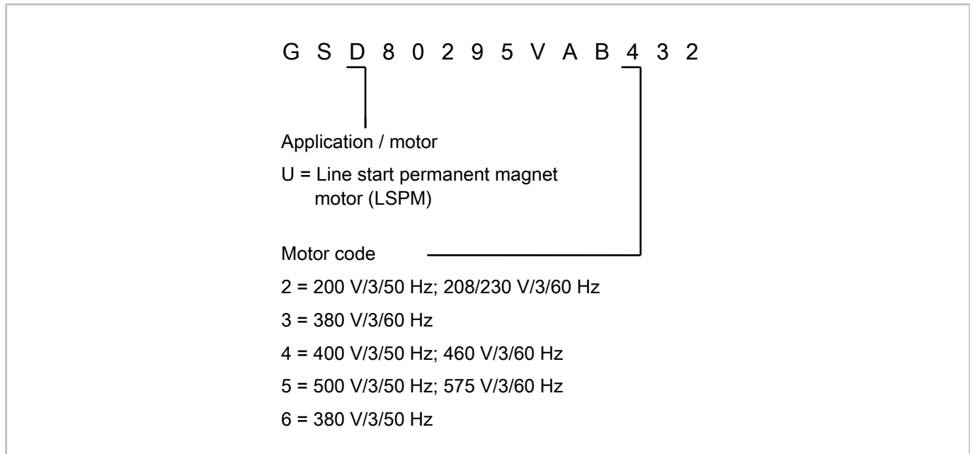
Fig. 10: Explanation of the motor codes for scroll compressors of the ORBIT series (example here: GSD)
