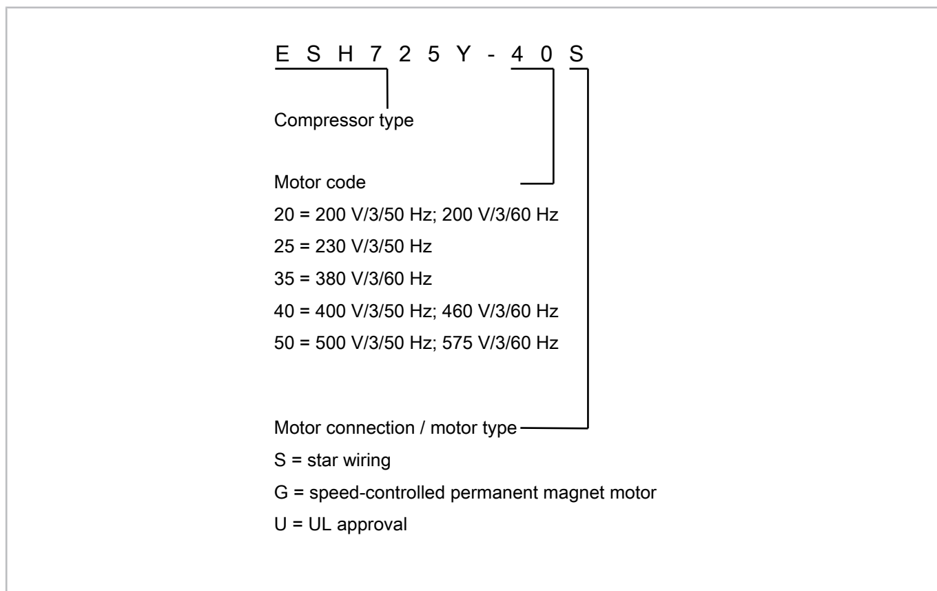
Fig. 11: Explanation of the motor codes for scroll compressors of the ESH7, ELH7 and ELA7 series (example here: ESH7)
